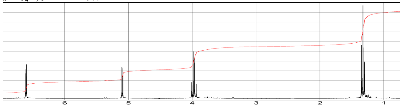
S-7 C 4 H 7 OBr 300MHz
